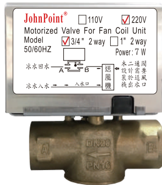
3/4" 2 way
