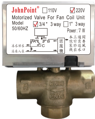
3/4" 3 way
